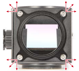
BFM II – seen from above. Use the screws for adjusting the thread.
